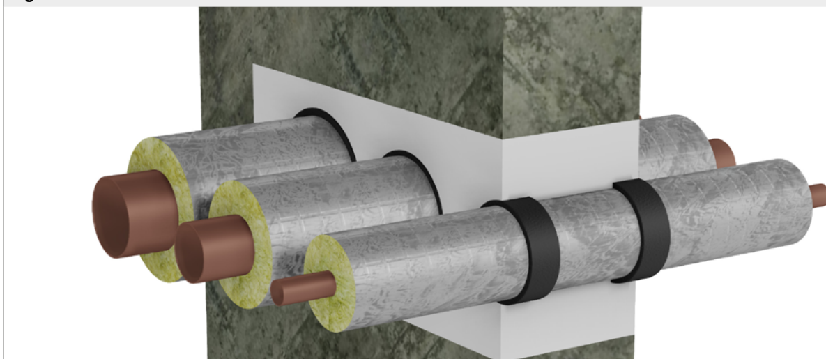
Figure 41. Thickness of GPG 130 mm
